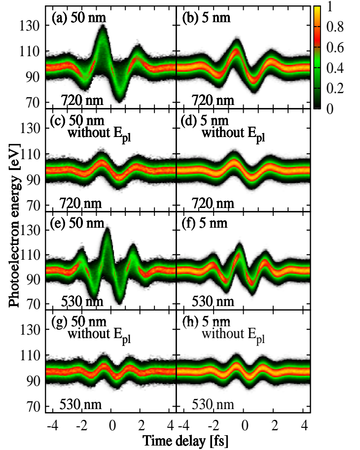
Figure 10. (Color online) Streaked spectra from Au nanospheres for streaking-pulse wavelengths of (a-d) 720 nm and (e-h) 530 nm, with radii of (a,c,e,g) 50 nm and (b,d,f,h) 5 nm. The spectra are normalized individually to their maximal yields. Results from full simulations that (a,b,e,f) include and (c,d,g,h) do not take into account the plasmonic field \vec{E}_{pl} [Eq. (4)].
