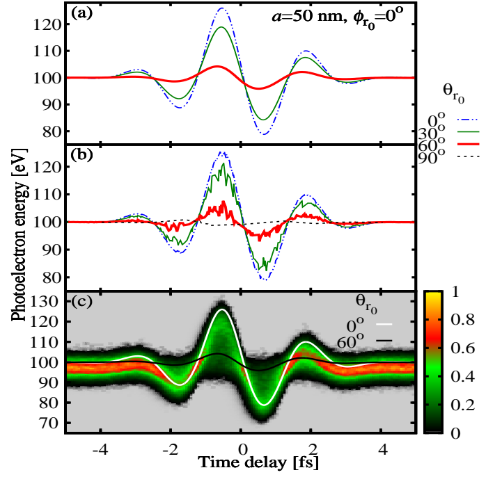
Figure 6. (Color online) Streaking curves and streaked spectra from 50 nm Au nanospheres. (a) Streaking curves for photoelectrons emitted from the Fermi level with emission direction \theta_{v_0} = 0^\circ for four emission latitudes \theta_{r_0} between the pole and equator on the nanosphere surface. (b) As (a) for randomized velocity directions \theta_{v_0} . (c) Simulated streaked spectrum and two streaking curves from release points ( r_0 = a, \theta_{r_0} = 0^\circ ) (white curve) and ( r_0 = a, \theta_{r_0} = 60^\circ ) (black curve). The spectrum is calculated for emission from the entire occupied conduction band, while the two streaking curves are calculated for emission from the Fermi level only. The spectrum is normalized to its maximal yield. For the two streaking curves the assumed emission direction is \theta_{v_0} = 0^\circ .
