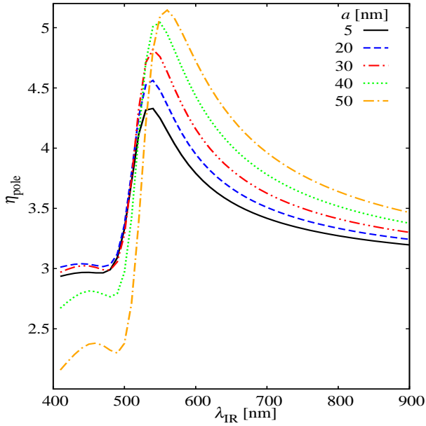
Figure 3. (Color online) Plasmonic-field enhancement at the poles of gold nanospheres of different radii a as a function of the wavelength \lambda_{IR}^{ctr} of the incident 10^{12} \text{ W/cm}^2 peak intensity pulse.
