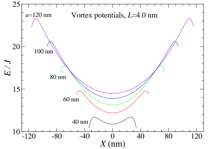
FIG. 3: Numerically determined vortex potentials, in units of the effective cell exchange constant J = 2AL , for circular Py nanodisks of thickness L = 4.0 nm and indicated radii, as found from the Lagrange constrained spin alignment relaxation. The vortex becomes unstable towards escaping from the disk in the regions of downward curvature.
