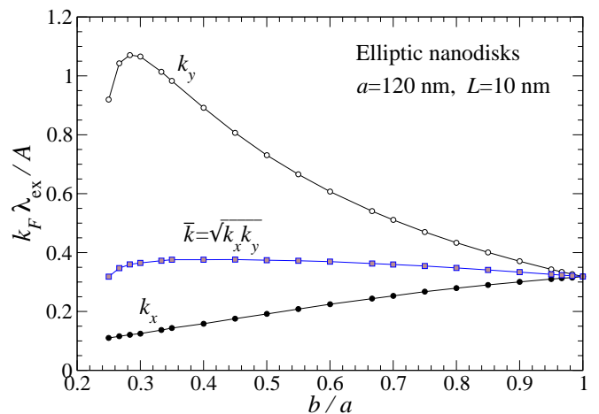
FIG. 6: Effective potential force constants versus geometric ellipticity b/a , for elliptic nanodisks of semi-major axis a = 120 nm, and thickness L = 10 nm. Results were found by Lagrange constrained spin alignment relaxation.
