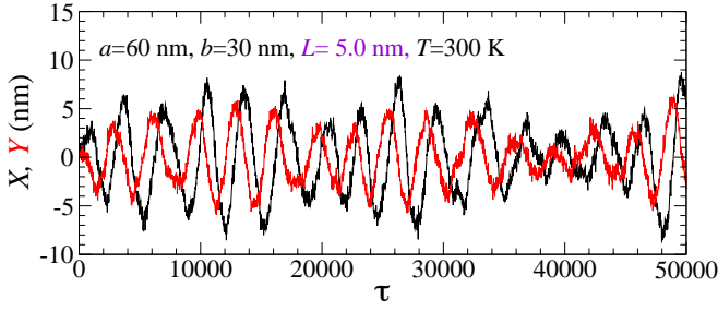
FIG. 9: Spontaneous vortex core motion caused by thermal fluctuations, as found by H2 integration of the LLG-Langevin equations (21) for a nanodisk with thickness L = 5.0 nm. The vortex was initiated at the disk center, X = Y = 0 . This graph shows only 1/5 of the total data generated and used subsequently for analysis of vortex statistics, corresponding to hundreds of gyrotropic periods.
