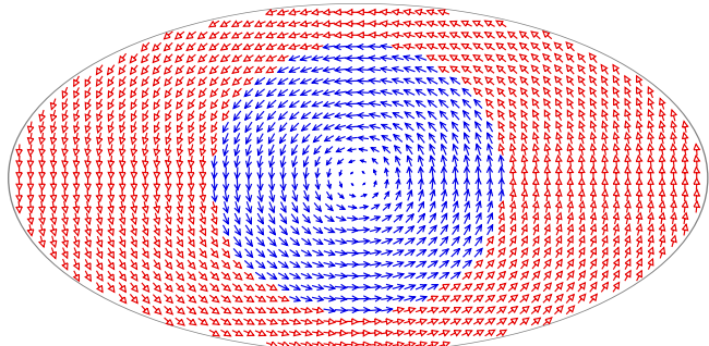
FIG. 1: The magnetization field \vec{M}(\mathbf{r}) = M_s \hat{m}(\mathbf{r}) of a vortex centered in a nanodisk with principal axes a = 60 nm, b = 30 nm, thickness L = 10 nm, from the spin alignment relaxation scheme for the micromagnetics model, Sec. 2.4. The cell size is a_{\text{cell}} = 2 nm. Arrows show only the in-plane projection, (m_x^i, m_y^i) . Blue line (red open) arrows indicate positive (negative) values of out-of-plane component m_z^i . The core, where m_z^i is larger, appears as a hole in this projection. Even though the system is elliptical, note that the core region remains close to circular.
