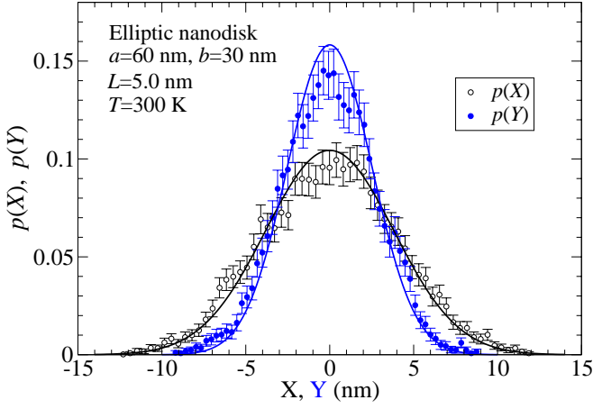
FIG. 12: Distributions of vortex core coordinates for the LLG-Langevin simulation in Fig. 9 with a = 60 nm, b = 30 , and thickness L = 5.0 nm. The solid curves are the theory expressions from Eq. (59) based on the Thiele theory for vortex motion, using force constants k_x = 0.1156 k_0 and k_y = 0.2657 k_0 from spin alignment relaxation, where k_0 = A/\lambda_{\text{ex}} .
