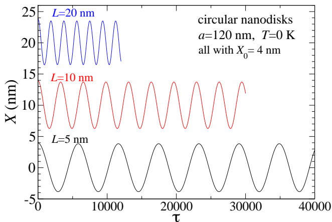
FIG. 4: Motions for one component of vortex position in circular nanodisks from RK4 integration of the LLG equations (shifted for clarity). The damping \alpha = 0.02 was turned off after dimensionless time \tau = 1000 . The periods can be calculated accurately from the undamped motion. Graphs of Y(\tau) are of the same amplitudes and frequencies but shifted a quarter of a period.
