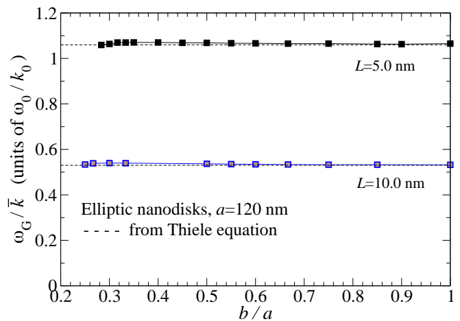
FIG. 8: Gyrotropic frequency magnitudes (from dynamics) scaled by mean force constants (from statics), versus geometric ellipticity b/a , for elliptic nanodisks with a = 120 nm and two different thicknesses. The results confirm the predictions from the Thiele theory, dashed lines from Eq. (43), using exchange length \lambda_{\text{ex}} = 5.3 nm, with no adjustable parameters.
