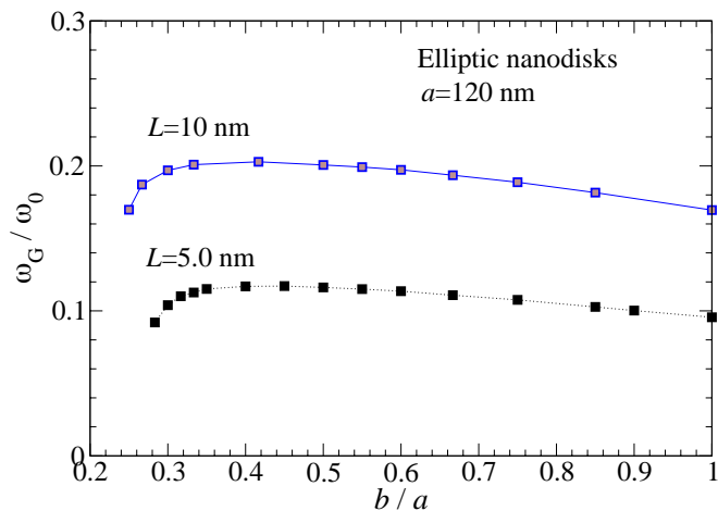
FIG. 7: Gyrotropic frequency magnitudes versus geometric ellipticity b/a , for elliptic nanodisks of semi-major axis a = 120 nm, and thicknesses L = 5.0 nm and L = 10 nm. Results were found by simulations of the LLG equations using RK4 integration. For L = 10 nm, compare the similar shape of the curve of \bar{k} in Fig. 6, as expected from \omega_G \propto \bar{k} in Eq. (43).
