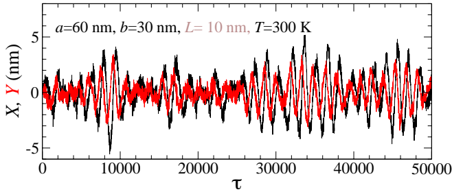
FIG. 10: Spontaneous vortex core motion caused by thermal fluctuations, for a nanodisk simulation identical to that in Fig. 9, but with double the thickness, L = 10 nm. Note the considerably smaller amplitude of gyrotropic oscillations, and the much higher frequency.
