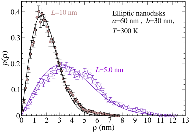
FIG. 11: The radial distribution of vortex core positions for the simulations in Figs. 9 and 10, with a = 60 nm, b = 30 , and thicknesses L = 5.0, 10 nm. Data out to final time \tau = 2.5 \times 10^5 was used. The solid curves are the theory expression (57), using force constants \bar{k} = 0.1753 k_0 for L = 5.0 nm and \bar{k} = 0.6832 k_0 for L = 10 nm, as obtained from spin alignment calculations, with force constant unit k_0 = A/\lambda_{\text{ex}} .
