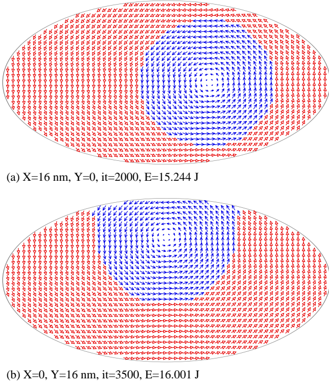
FIG. 2: Vortex structures for an elliptical nanodisk with a = 60 nm, b = 30 nm, L = 10 nm, using cell size a_{\text{cell}} = 2.0 nm in the spin alignment relaxation scheme, including a Lagrange constraint on position. (a) Vortex is held at X = 16 nm, Y = 0 , resulting in total energy E = 15.244J after 2000 iterations. (b) Vortex is held at X = 0 , Y = 16 nm, resulting in total energy E = 16.001J after 3500 iterations. Compare Fig. 1, where X = Y = 0 and the energy is lower.
