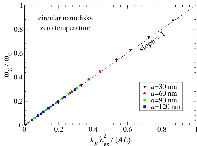
FIG. 5: Vortex gyrotropic frequency magnitudes from RK4 (dynamics) simulations for circular nanodisks, with thicknesses ranging from L = 2.0 nm to 20 nm, and indicated disk radii, versus force constants scaled by disk thickness, obtained from Lagrange constrained spin alignment (static) simulations. The dashed line is the theoretical result (43) from the Thiele equation.
