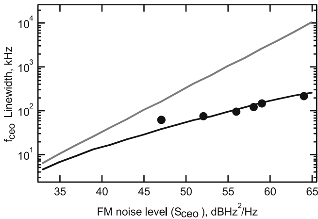
FIGURE 10 FWHM line width of f_{\text{ceo}} vs. the one-sided power spectral density in frequency noise units. Black line : numerically calculated linewidth for a 7-kHz roll-off. Gray line : calculated linewidth for an infinite roll-off ( = \pi S_{\text{ceo}} ). Solid markers : measured linewidths, \Delta f_{\text{ceo}} , vs. measured frequency noise, S_{\text{ceo}}(0)
