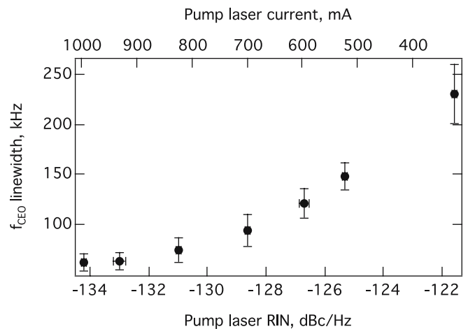
FIGURE 4 FWHM linewidth of f_{ceo} , using Lorentzian line shape fitting, as a function of pump laser current and the corresponding relative-intensity noise
