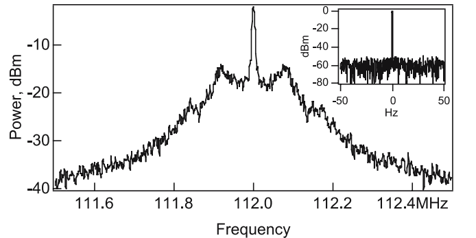
FIGURE 14 Field spectrum of the phase-locked f_{\text{ceo}} beat at 3-kHz resolution bandwidth. Inset: phase-locked f_{\text{ceo}} beat at 0.3-Hz resolution bandwidth and centre frequency offset to 0 Hz
