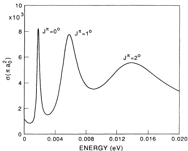
FIG. 8. Converged total elastic cross section for e^- -Cs scattering. The peaks from left to right correspond to the 6s6p\ ^3P_J^o , J=0,1,2 shape resonances, respectively.
