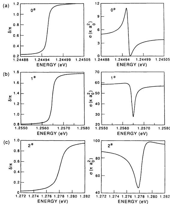
FIG. 5. Highly resolved eigenphase sums (modulo \pi , left) and partial cross sections for the 6p^2\ ^3P^e shape resonances: (a) J=0 , (b) J=1 , (c) J=2 . The calculation includes the Buttler correction and the dielectronic term.
