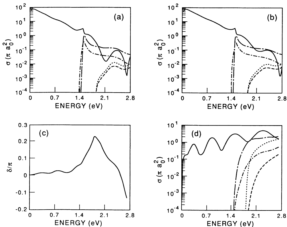
FIG. 3. Results without Buttlet correction and with dielectronic term for two J^\pi symmetries: (a) partial cross sections for J^\pi=0^e and 15 continuum orbitals per channel; (b) partial cross sections for J^\pi=0^e and 24 continuum orbitals per channel; (c) eigenphase sum (modulo \pi ) for J^\pi=5^e and 24 continuum orbitals per channel; (d) partial cross sections for J^\pi=5^e and 24 continuum orbitals per channel. The partial cross sections are for elastic scattering (—), 6s-6p_{1/2} excitation (-.-.-), 6s-6p_{3/2} excitation (---), 6s-5d_{3/2} excitation (- - -) and 6s-5d_{5/2} excitation (. . .). For converged results see Figs. 4(a) and 4(k).
