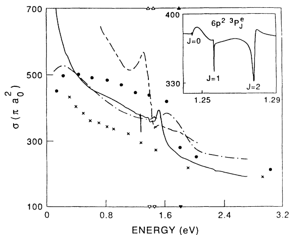
FIG. 7. Converged total cross section for low-energy e^- -Cs scattering compared with published results. Theory: present work (—), Ref. [10] (— · — · —), Ref. [17] (---), Ref. [20] (····). Experiment: Ref. [4] (×). The 6p_{1/2,3/2} and 5d_{3/2,5/2} thresholds are marked by the small triangles. The inset (same units as main plot) shows the 6p^2\ ^3P_J^e , J=0,1,2 resonances, which are not fully resolved in the main plot. The large cross sections we obtain at the lowest shown energies correspond to the strong resonance enhancement of the elastic cross section close to threshold due to the resonances shown in Fig. 8. Our calculation includes the Buttke correction and dielectronic term.
