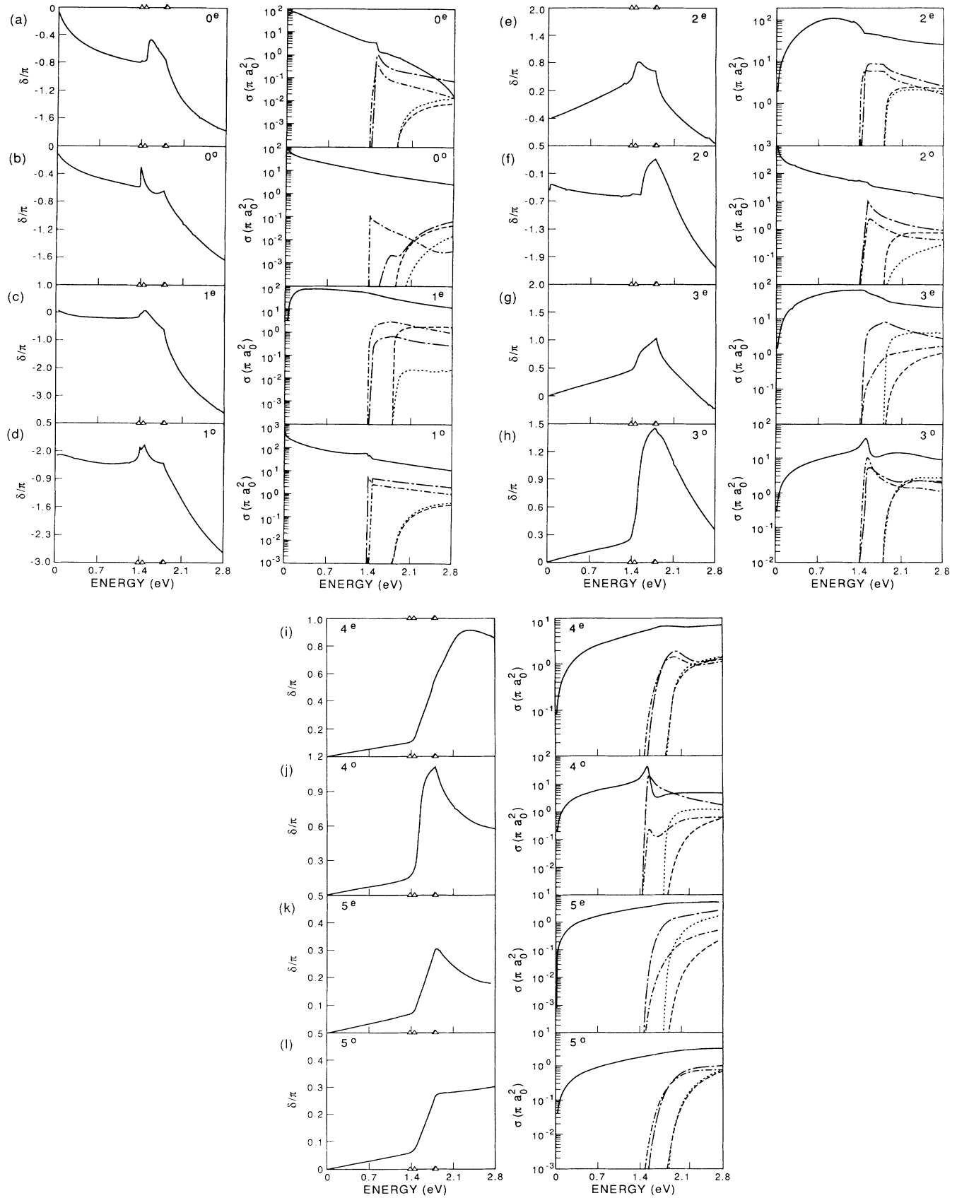
FIG. 4. Eigenphase sums (modulo \pi , left) and partial cross sections (right) calculated with the Buttke correction and the dielectronic term for J \leq 5 . Solid and interrupted lines as in Fig. 3. The J^\pi symmetries are (a) 0^\circ , (b) 0^\circ , (c) 1^\circ , (d) 1^\circ , (e) 2^\circ , (f) 2^\circ , (g) 3^\circ , (h) 3^\circ , (i) 4^\circ , (j) 4^\circ , (k) 5^\circ , (l) 5^\circ . For the eigenphase sums the small triangles indicate the 6p_{1/2,3/2} and 5d_{3/2,5/2} thresholds.
