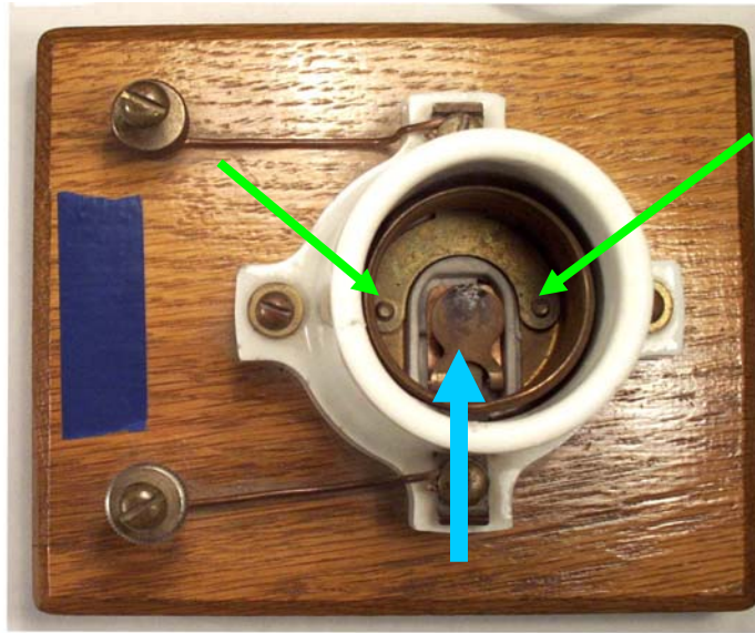
Figure 6: Socket similar to those used for Activity 3: Getting Connected . The green arrows indicate the locations of the point where the base is connected to the side. The large blue arrow indicates the tab on the base where many students tried to connect both wires from the Christmas tree light.
