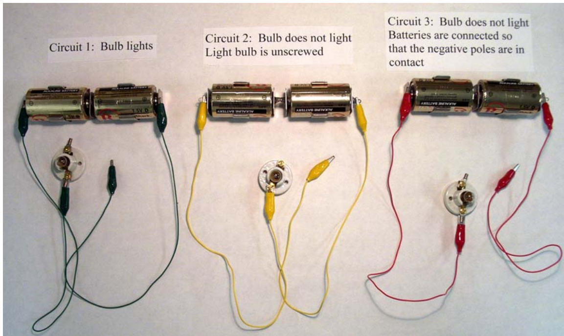
Figure 3: Circuits for Activity 2: That Glowing Feeling .
