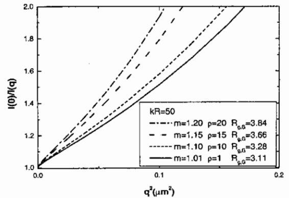
Fig. 1. Guinier plot of calculated Mie scattering data for spheres with size parameter kR = 50 and different refractive indices m . To give the plot some physical relevance we assume \lambda = 0.5 \mu\text{m} , thus R = 3.98 \mu\text{m} and R_g = 3.08 \mu\text{m} .
