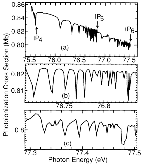
FIG. 1. Photoionization spectrum of He 1P^\circ states: (a) below the N = 5 and 6 thresholds (IP 5 , IP 6 ), (b) magnification of the high- n region below the N = 5 threshold, (c) magnification of the high- n region below the N = 6 threshold.
