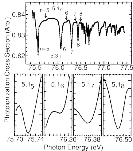
FIG. 2. Photoionization spectrum of He convoluted with experimental resolution of 6 meV below the N = 5 and 6 thresholds. Resonances labeled 5, 1_n are magnified underneath. Note that the dots are calculated points and the solid lines simply join them smoothly.
