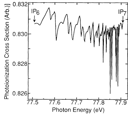
FIG. 4. Photoionization spectrum below the N = 7 threshold.
