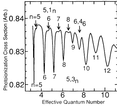
FIG. 3. Photoionization spectrum below the N = 5 threshold as a function of effective quantum number.
