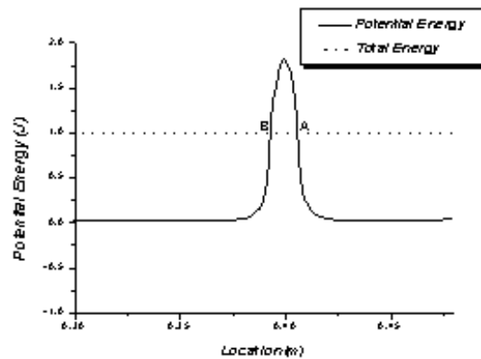
Figure 10: The magnets repel and the total energy is less than the maximum potential energy.
