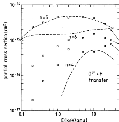
FIG. 10. Partial cross sections for transfer into O^{7+} n=4, 5, and 6 orbitals in O^{8+} + H collisions. Results of the present AO study are indicated by open squares, results of the multistate MO investigation (Ref. 4) by dashed lines.
